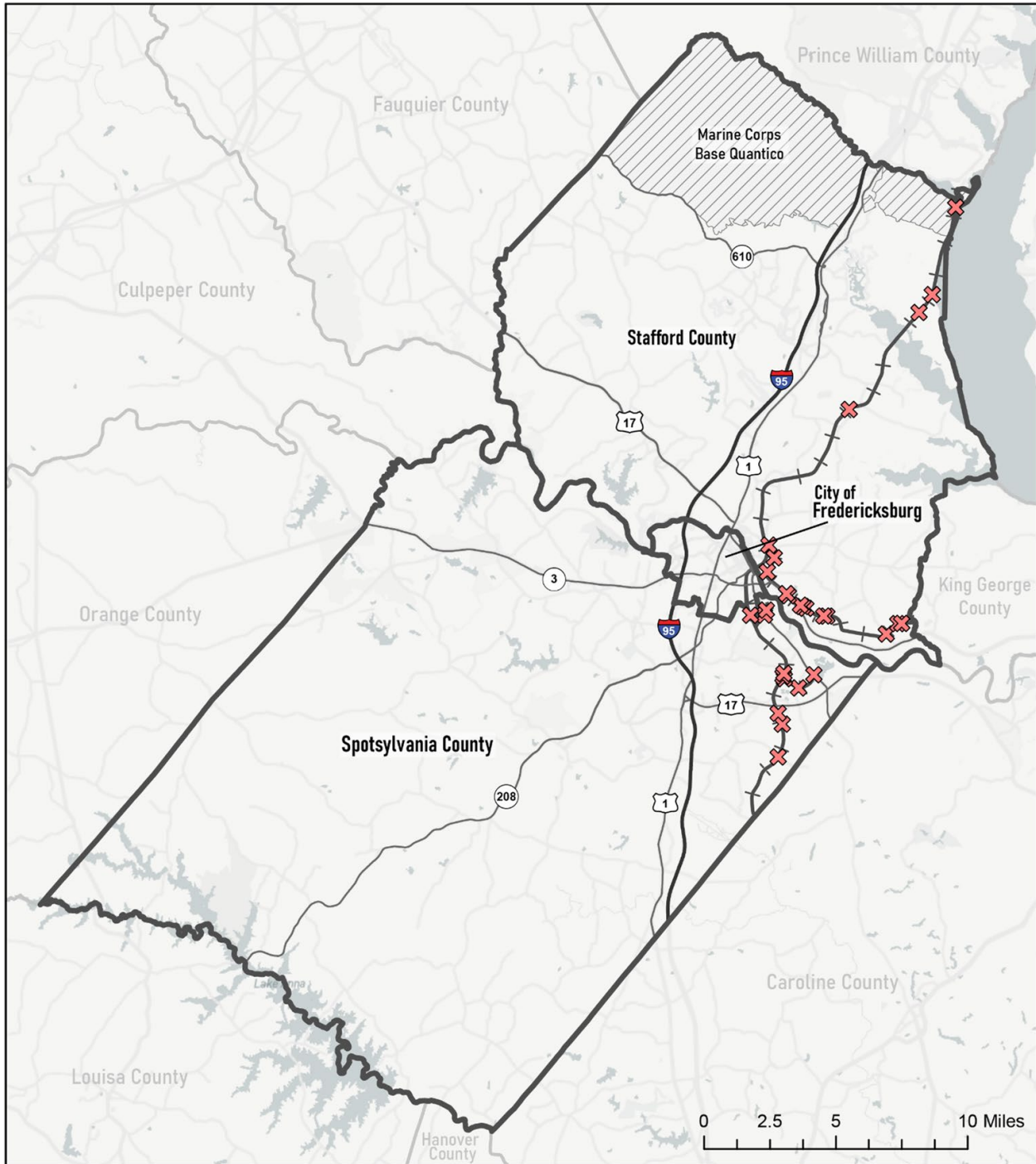
Map 5.9: Regional Rail System and Active At-Grade Public Rail Crossings
