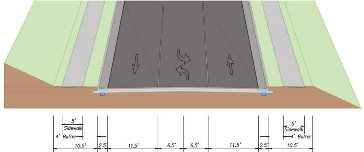
Typical Section
