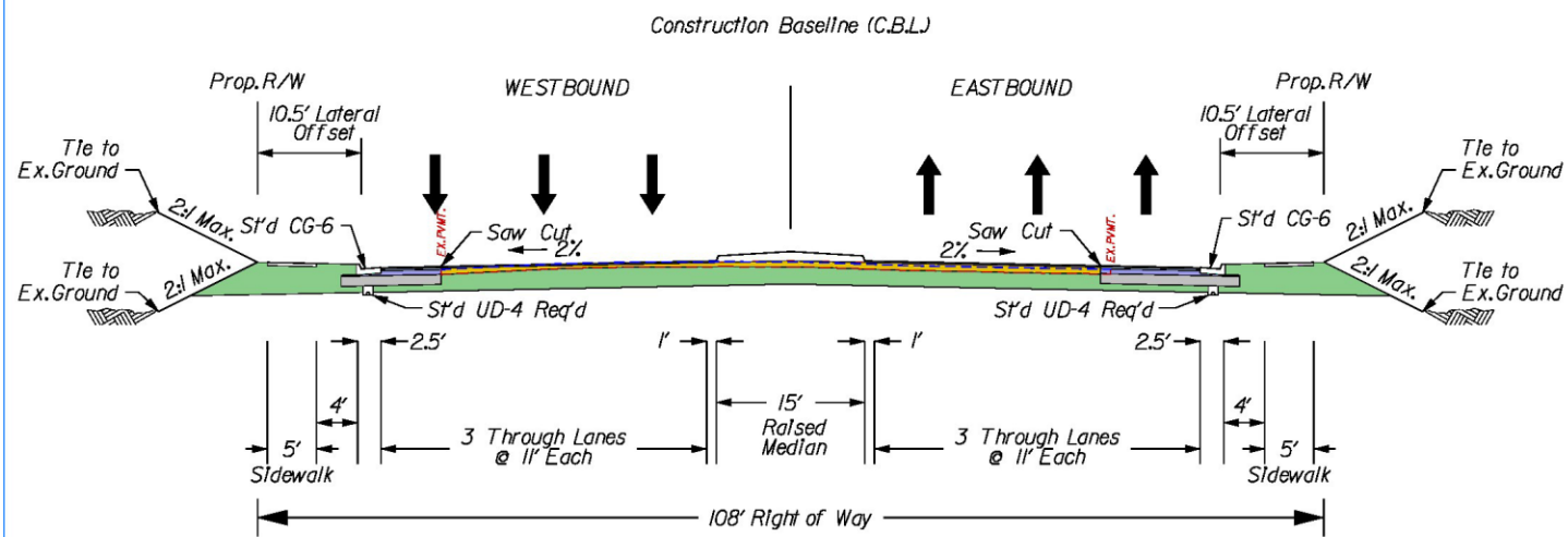
Typical Section
